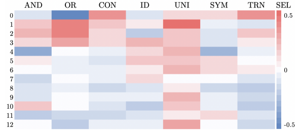
Figure 3: Probe selectivity computed by Definition 1.
